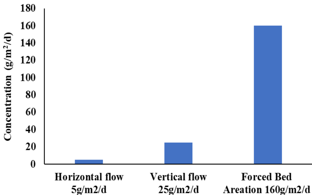
Figure 12: Comparison of oxygen transfer rates in CWs (Source: Personal communication Sh. Ganges Reddy, dated- August 22, 2023)
