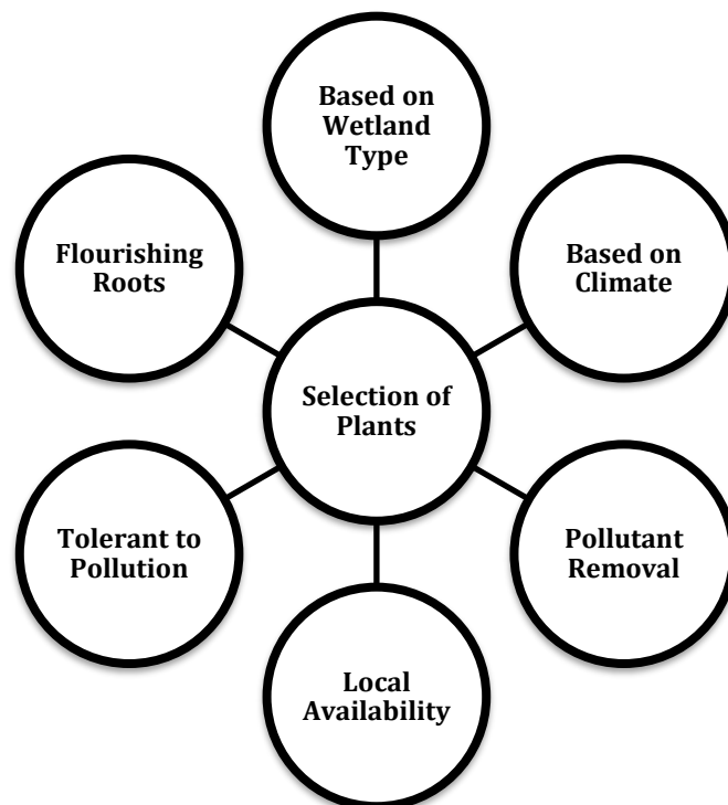
Figure 16: Factors to be considered for selection of plants for constructed wetlands
