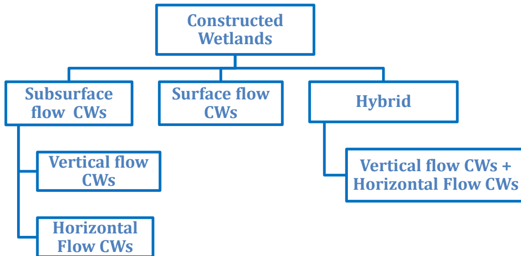
Figure 1: General classification of Constructed wetlands
