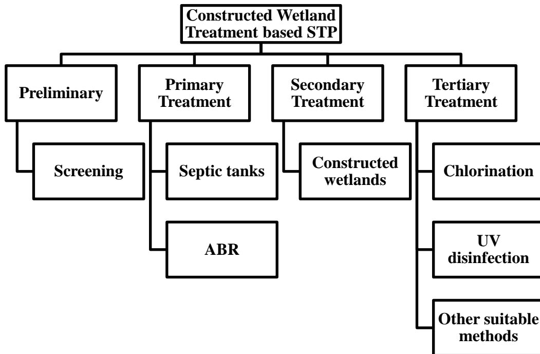
Figure 9: Process flow of CWs based STPs
