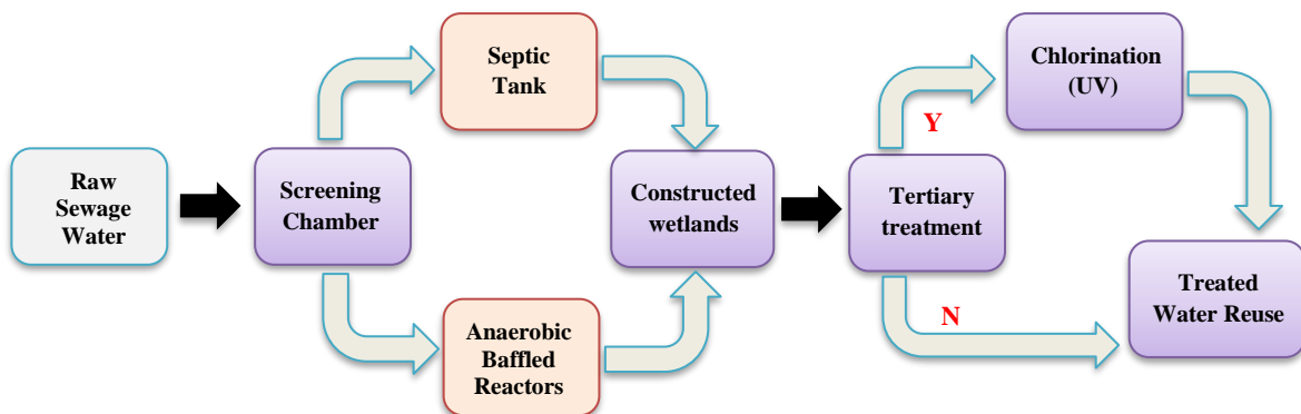
Figure 11: Integrated treatment set up with CWs
