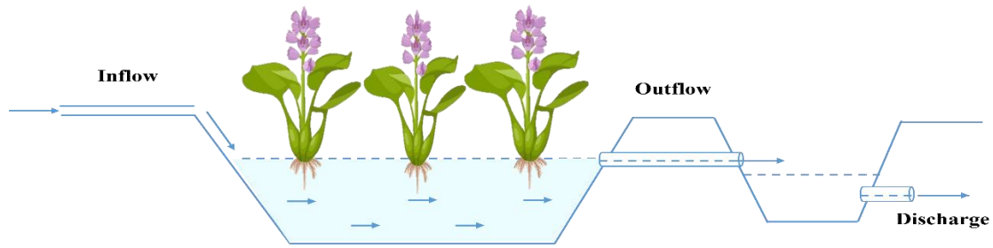
Figure 4: Basic design configuration of free surface water constructed wetlands
