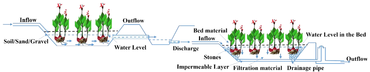
Figure 5: Basic design configuration of hybrid constructed wetlands
