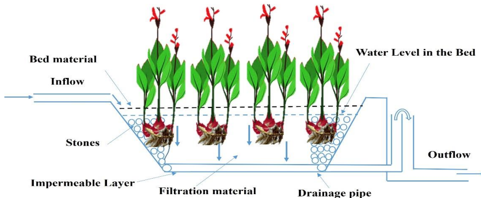
Figure 2: Basic design configuration of vertical flow constructed wetlands
