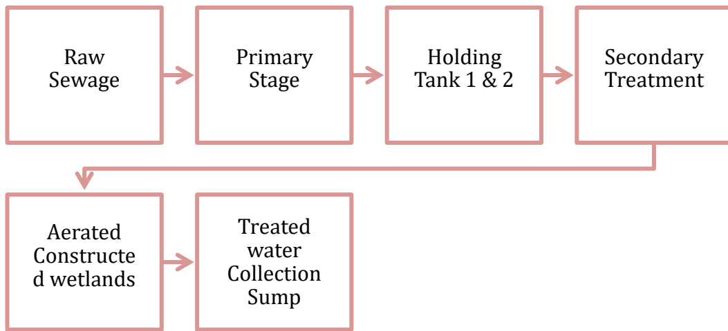
Figure: Process flow diagram
