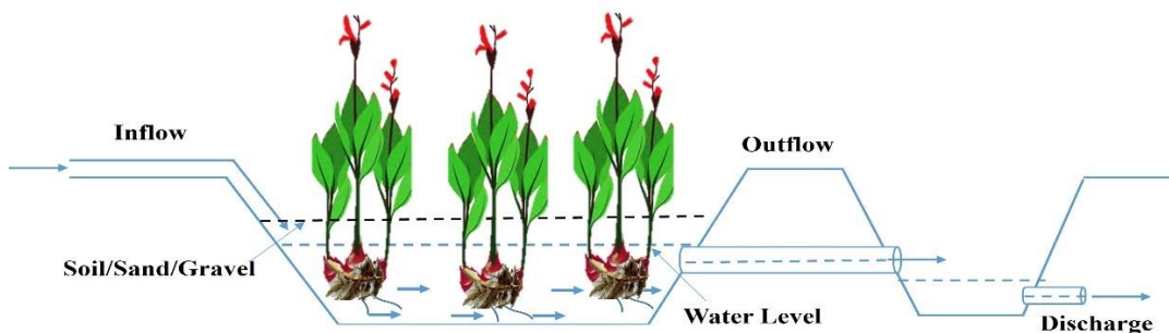
Figure 3: Basic design configuration of horizontal flow constructed wetlands
