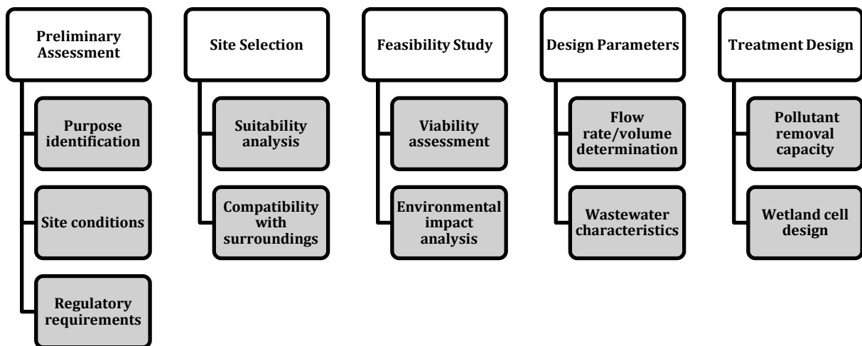
Figure 7: Basic strategy for selection of constructed wetlands
